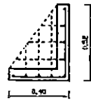
DETAIL A (ferrillage)
